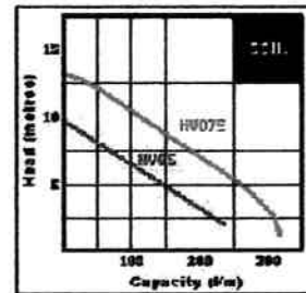
PUMP PERFORMANCE CURVES HYFLOW SERIES PUMPS
