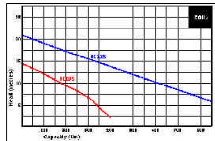
SEWAGE PUMP PERFORMANCE CURVES HYFLOW SERIES PUMPS
