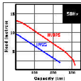
VORTEX PUMP PERFORMANCE CURVES HYFLOW SERIES PUMPS
