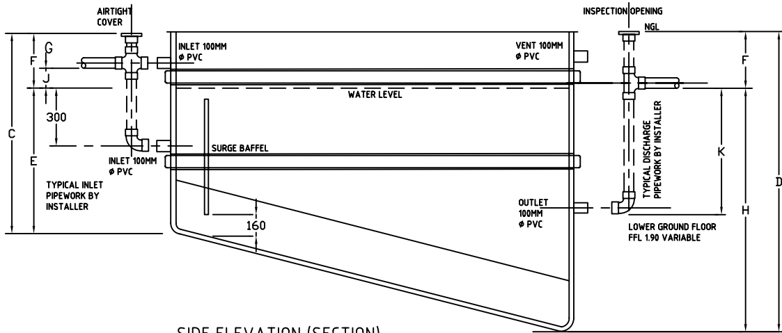
SIDE ELEVATION (SECTION)
